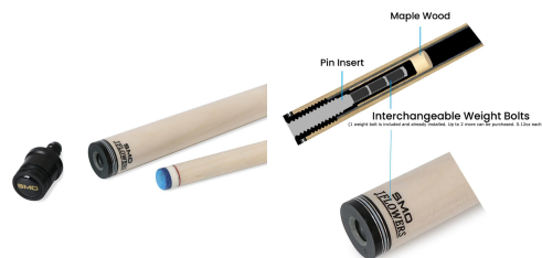
SMO-Wood-Shaft-Interchangeable-Weight-Bolts-0.12oz-Each-scaled
